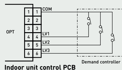
Indoor unit control PCB
