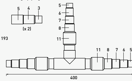
Discharge piping
