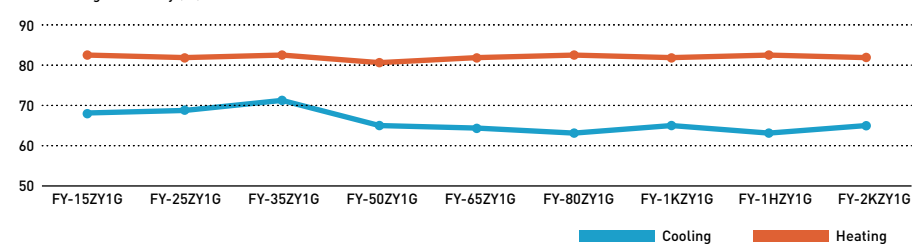
Heat exchange efficiency [%].
