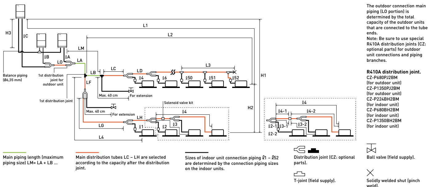
Ranges that apply to refrigerant piping lengths and to differences in installation heights
