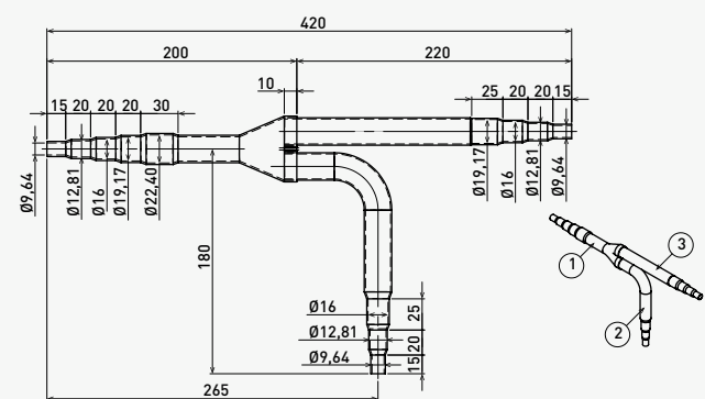
Liquid piping
