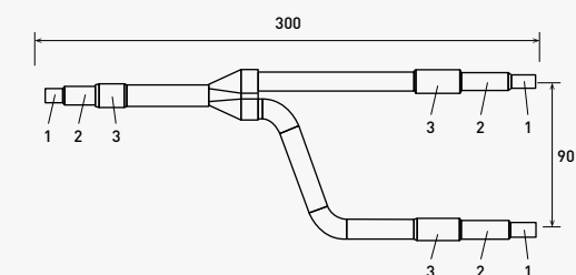
Liquid piping
