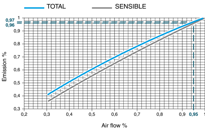
Diagram 1 - Cooling emissions
