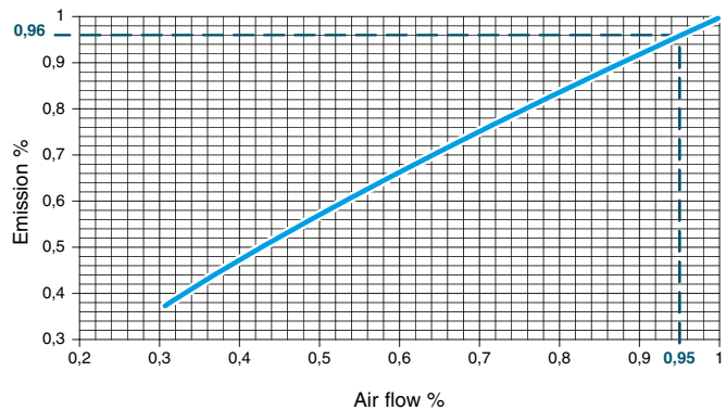
Diagram 2 - Heating emission
